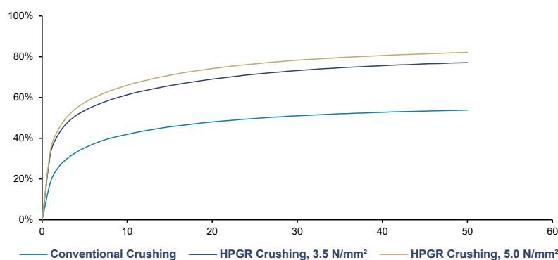
Leach Recovery by Technology, 0–50 Days
