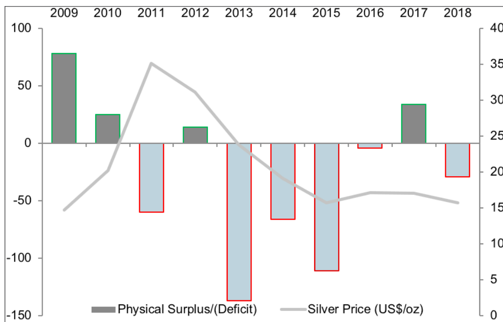
Figure 1: Silver Physical Surplus/Deficit
